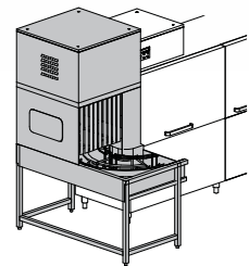
EVO: DRA184MC 4,5 kW Electric DRA189MC 9 kW Electric PRO: DRA184MT 4,5 kW Electric DRA189MT 9 kW Electric DRA18VMT Steam Asciugature ad angolo a 180° Dryer with arc 180°
